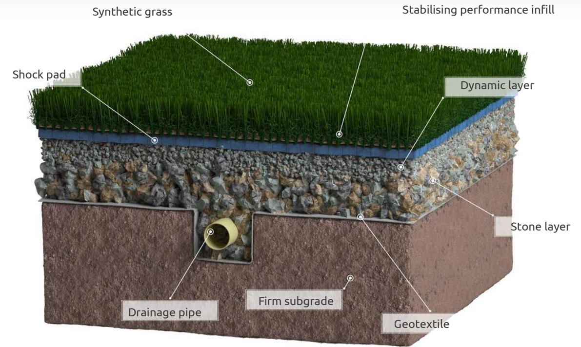
Typical PST Sport pitch base shown above
